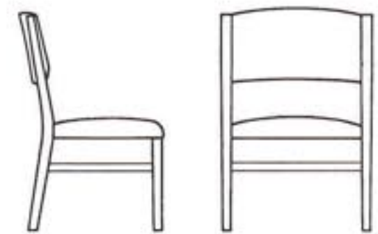
743 Arm Chair 31.5"H, 22"W, 24.5"D
