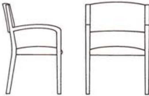
740 Arm Chair 31.5"H, 22"W, 24.5"D
